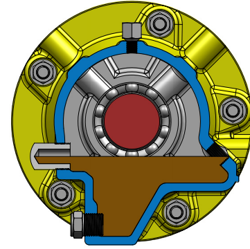
Non-overfilling design
