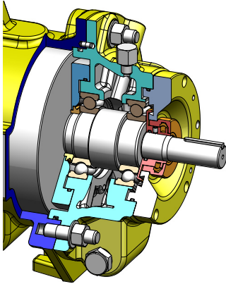
Standard design
