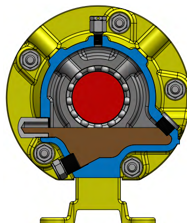
Non-overfilling design
