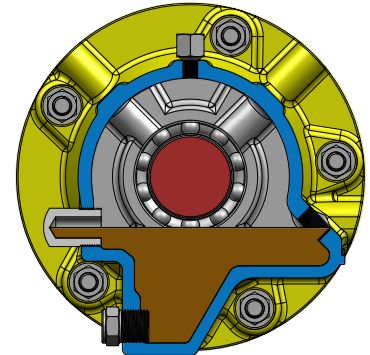
Non-overfilling design
